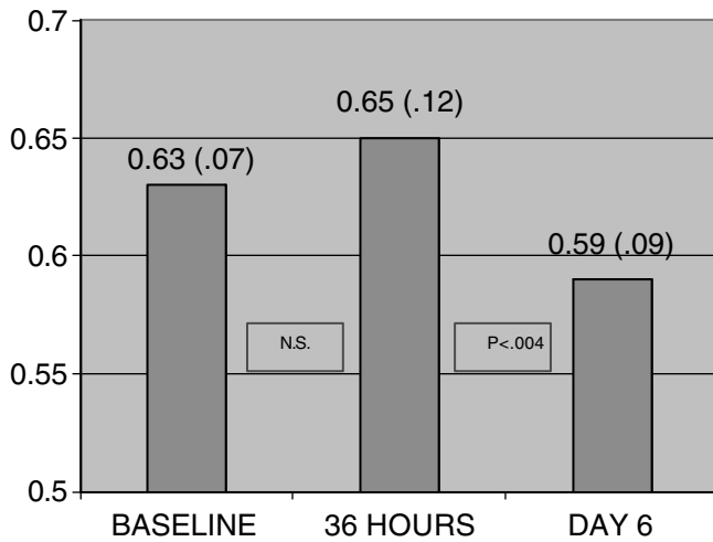
Figure 3. Mean performance on the ImPACT reaction time composite at baseline, 36 hours postinjury, and 6 days postinjury. Standard deviations are in parentheses. A lower score indicates better (faster) performance. Pairwise comparisons are provided between baseline and 36 hours and between 36 hours and day 6. Mildly concussed athletes show no initial change followed by better than baseline performance at day 6.
